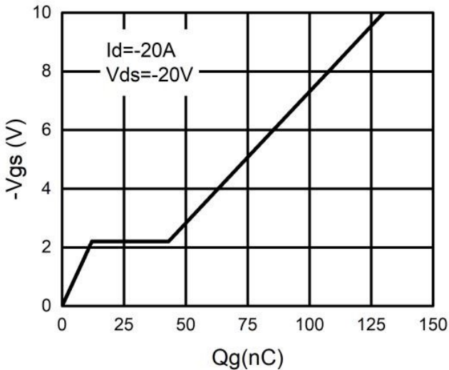
Fig.5 - Gate charge
