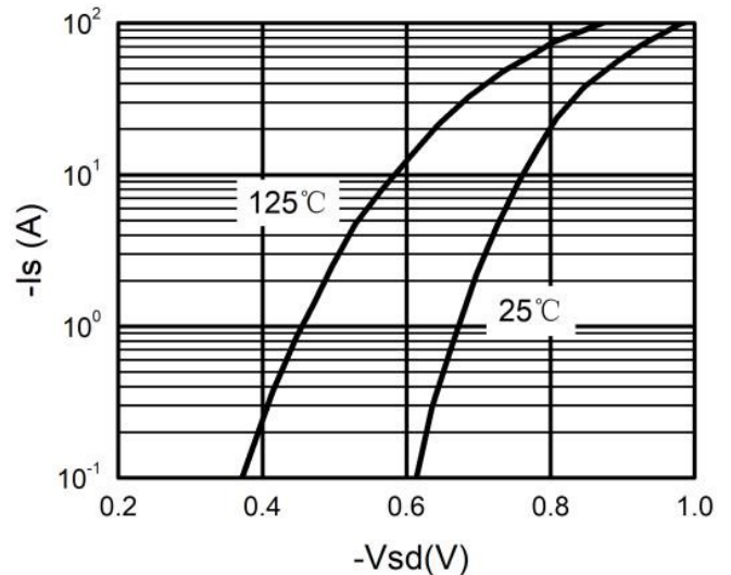
Fig.6 - Forward Characteristic
